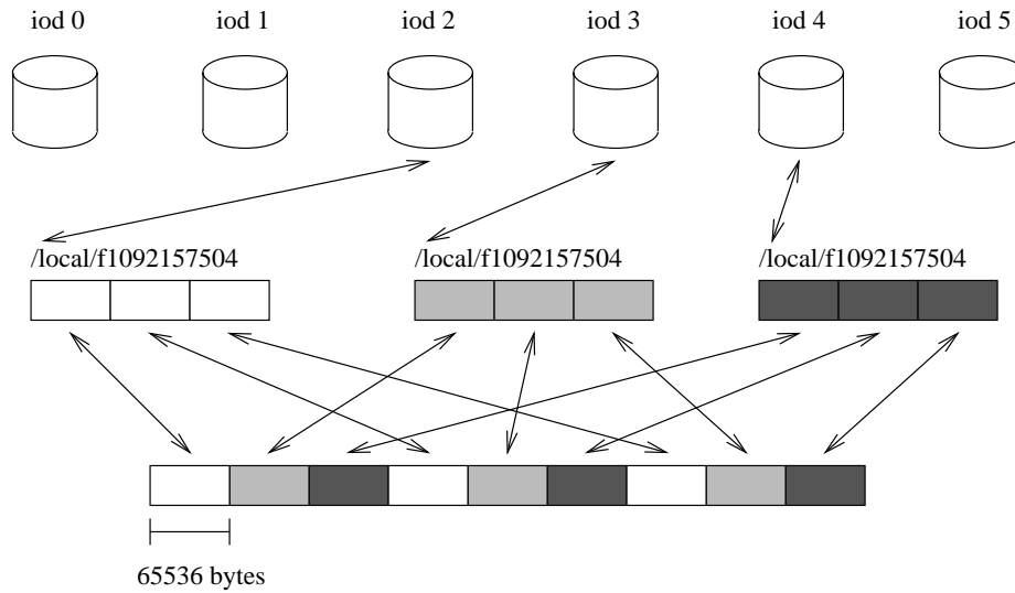
Figure 1: File-stripping example
